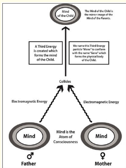
Figure 3: Role of Quantum mechanics in the formation of mind in a newly created human being.
