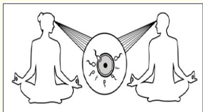
Figure 1: Influence of the EME of the minds of the parents on the activity of the sperm and ovum.
