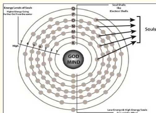
Figure 4: Role of Quantum mechanics in the formation of soul in a newly created human being.
