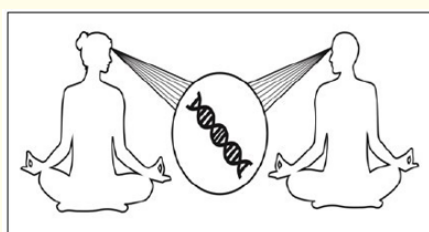
Figure 2: Influence of the EME of the minds of the parents on the Chromosome -> DNA -> Gene.
