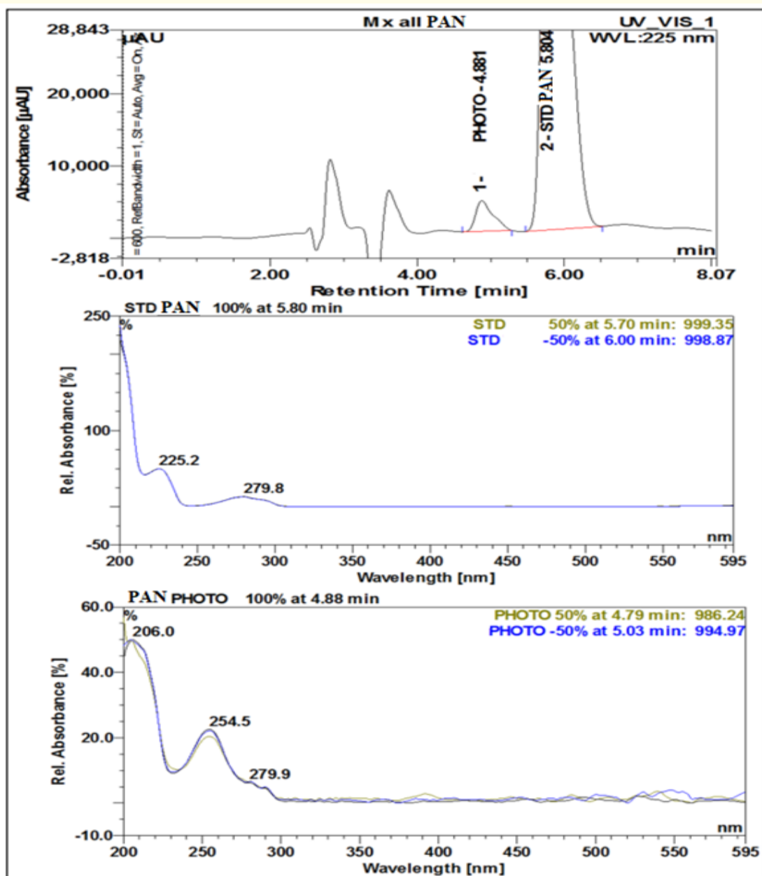
Figure 4: HPLC chromatogram and PDA absorption spectra of: A) Standard PAN and B) Photo degradant of PAN.
