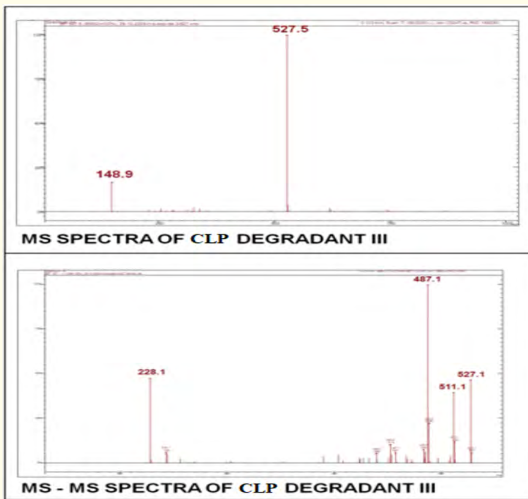
Figure 8: Mass spectral details of CLP degradant III.
