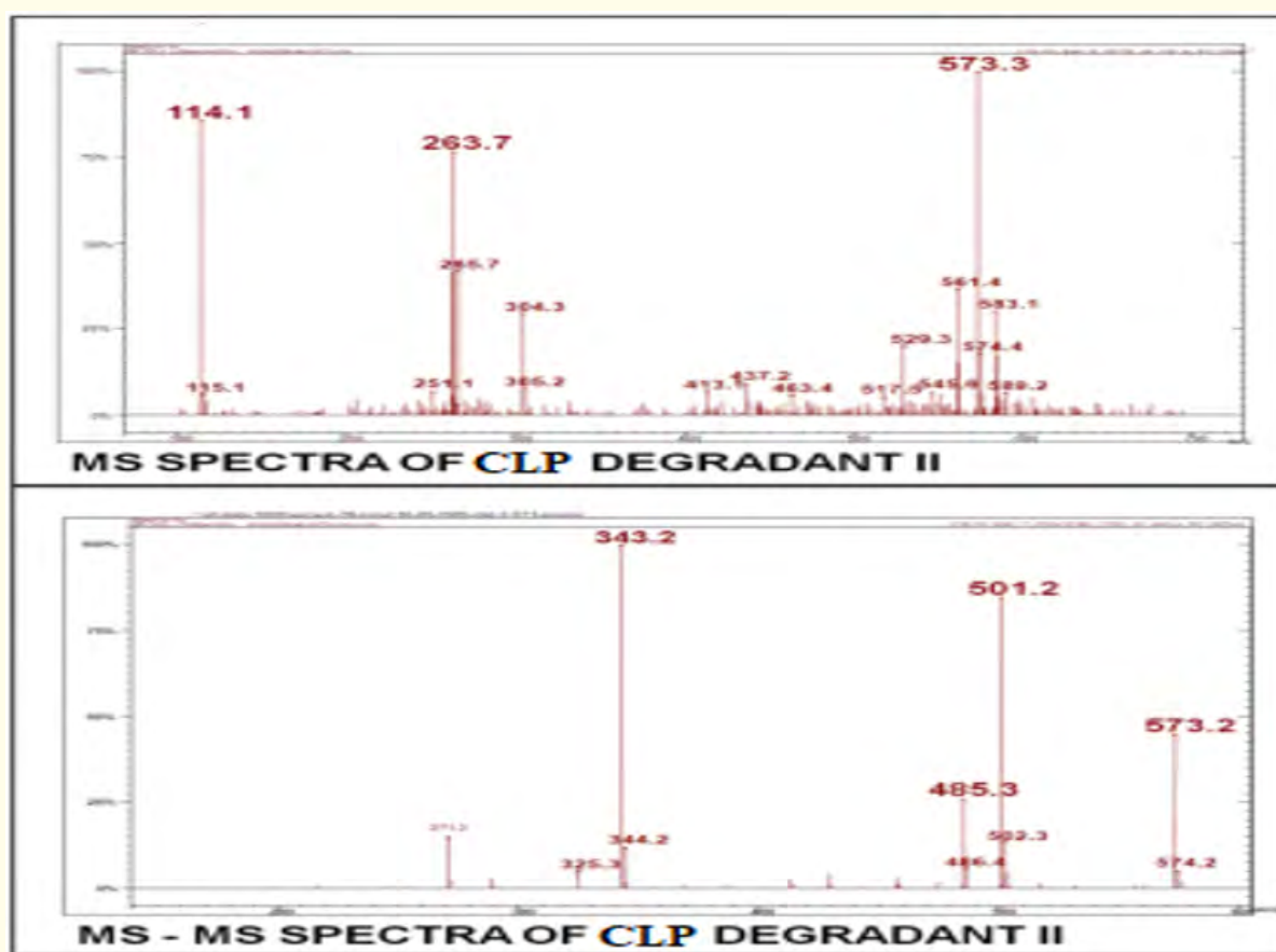
Figure 7: Mass spectral details of CLP degradant II.
