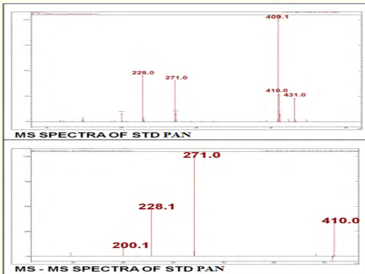
Figure 9: Mass spectra of standard PAN.
