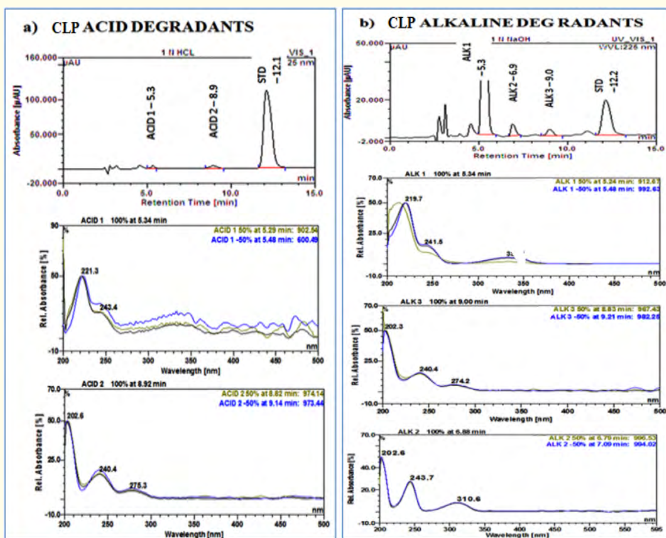
Figure 3: HPLC chromatogram and PDA absorption spectra of: A) Acid degradants of CLP and B) Alkaline degradants of CLP.
