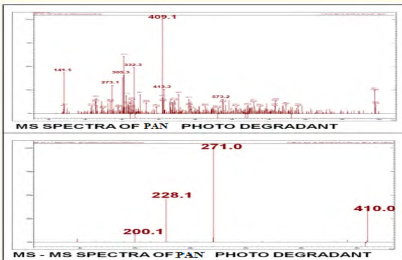
Figure 10: Mass spectra of PAN photo degradant.
