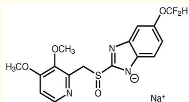
Figure 1B: Structure of pantoprazole sodium.
