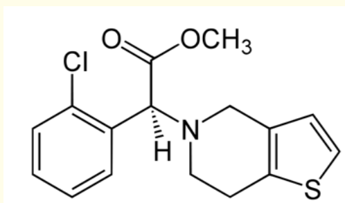
Figure 1A: Structure of clopidogrel.
