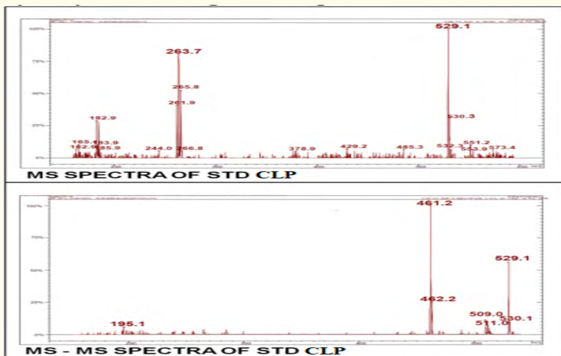
Figure 5: Mass spectral details of standard CLP.
