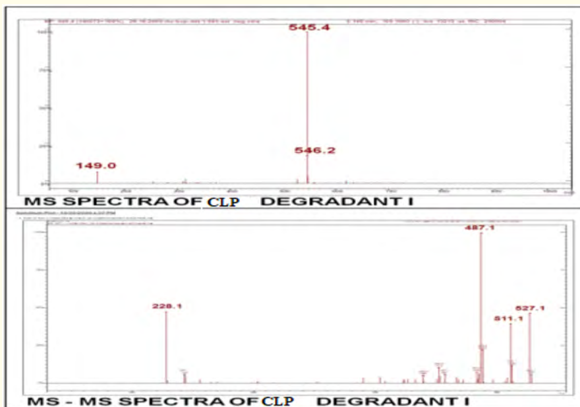
Figure 6: Mass spectral details of CLP degradant I.
