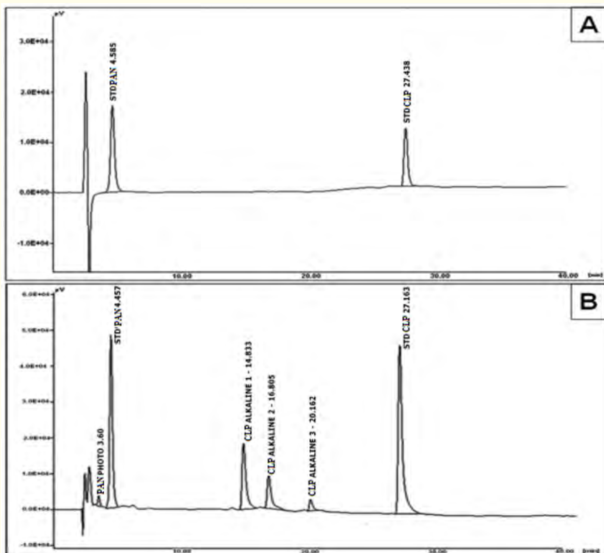
Figure 2: HPLC chromatogram of (A) Standard clopidogrel and pantoprazole hydrochloride (B) Degradants of clopidogrel and pantoprazole hydrochloride.
