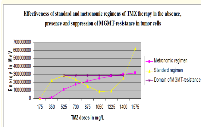
Figure 5: Shows the energy yield in standard and metronomic regimens of TMZ therapy in the absence, presence and suppression of MGMT-resistance in tumor cells.
