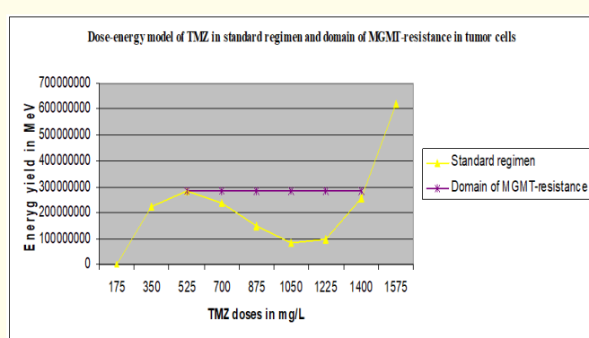
Figure 3: Shows energy yield by TMZ doses and the domain of MGMT-resistance in standard regimens.
