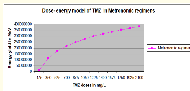
Figure 2: Shows the increase of energy yield by increasing TMZ doses in metronomic regimens expressing the non-existence of MGMT-resistance.
