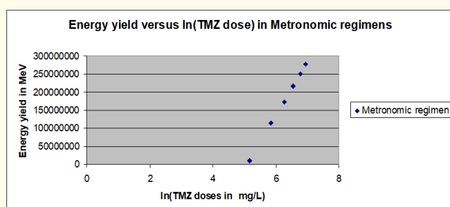
Figure 1: Shows a scatter plot expressing perfect correlation ( r = 1 ) between \ln (TMZ dose) and energy yield in metronomic regimens.
