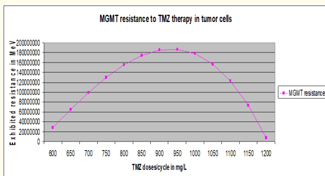
Figure 4: Shows the increase in MGMT-resistance to TMZ therapy in tumor cells to its maximum at 6.74 mg/kg bw/day (943.55 \mu\text{g/mL} ) and its decrease by increasing TMZ dose/day until being suppressed due to MGMT depletion in tumor cells.
