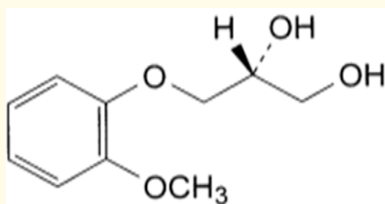
Figure 1: Chemical structure of guaifenesin.
