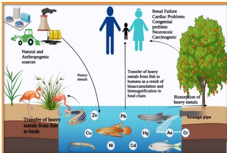
Figure 2: Heavy metal intake via the food chain.
