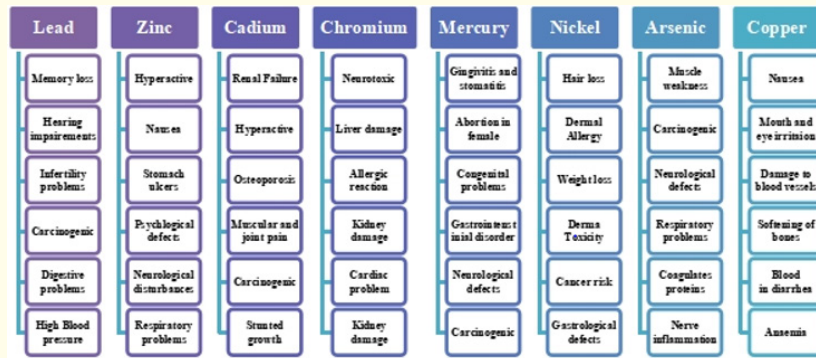
Figure 3: Effect of Heavy metals on human health.
