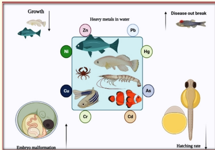
Figure 1: Impact of heavy metals on the aquatic health.
