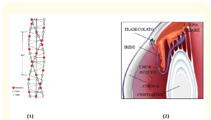
Figure 2: 1) Collagen structure.
