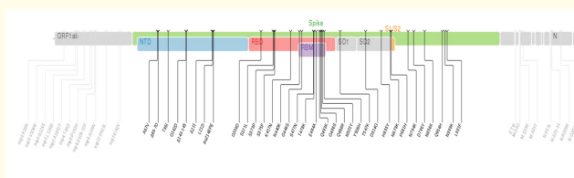
Figure 3: The Genomic Sequence in Omicron which has a high rate of mutation compares with Delta.
