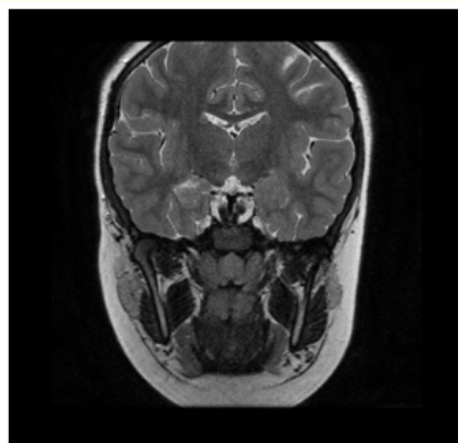
Figure 3: NMR examination.
