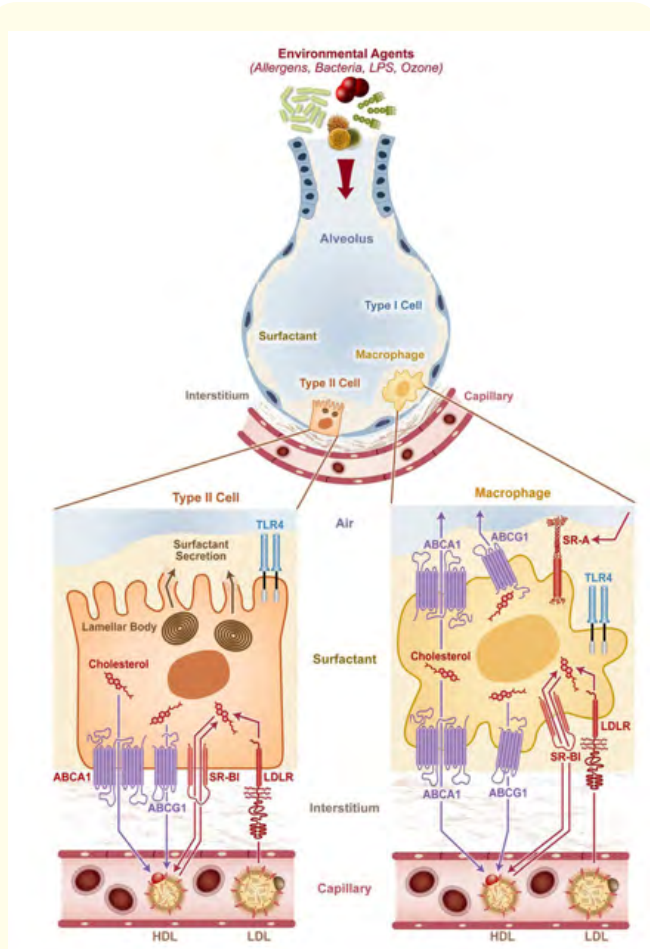
Figure 1: Demonstrating cholesterol trafficking influences multiple cell types in the lung.
