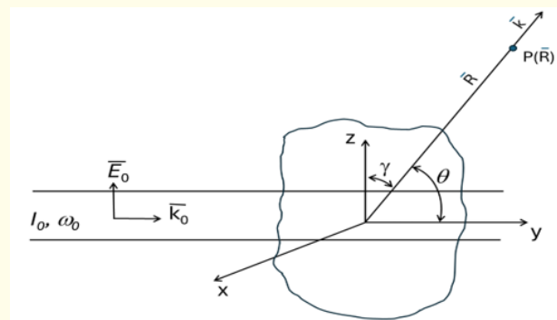
Figure 1: Is an experimental scheme for detecting scattered radiation. The laser beam propagates along the Y axis and is polarized along the Z axis; \omega , I_0 is the angular frequency and intensity of the laser radiation. The scattered radiation is recorded at the point P, the polar coordinates of which are R, \theta , \gamma . \theta is the angle between the direction of propagation of the light beam and the direction of propagation of the scattered radiation. The distance R is chosen in such a way as to avoid direct laser radiation hitting the photodetector.
