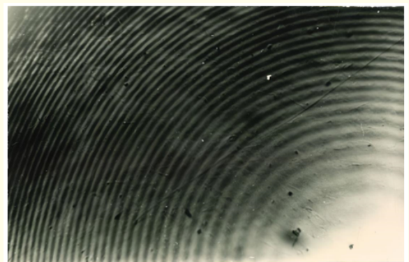
Figure 4: Is the result of interference of a diverging light beam with a light beam with a flat wavefront.
