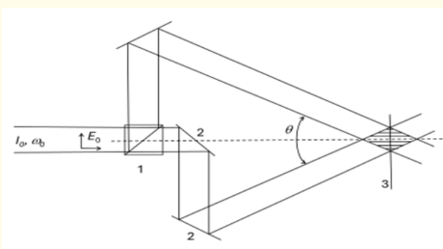
Figure 2: Experimental scheme for detecting radiation interference. The laser beam is divided into two equal parts using a beam-splitting cube -1. Using the mirror - 2 system, the two beams obtained intersect with each other ; \omega , I_0 is the angular frequency and intensity of the laser radiation. \theta is the angle at which the beams intersect. The interference pattern in the area of beam intersection is recorded on a photographic plate - 3.
