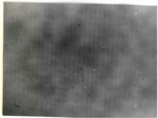
Figure 3: Is the result of interference of two flat intersecting laser beams recorded on a photographic plate.
