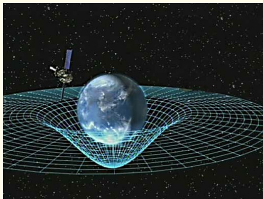
Figure 2: Propagation of gravitational waves.
