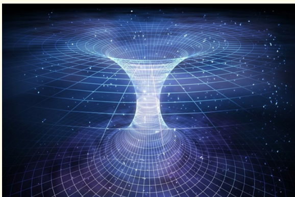
Figure 1: Interaction of gravitational energies.
