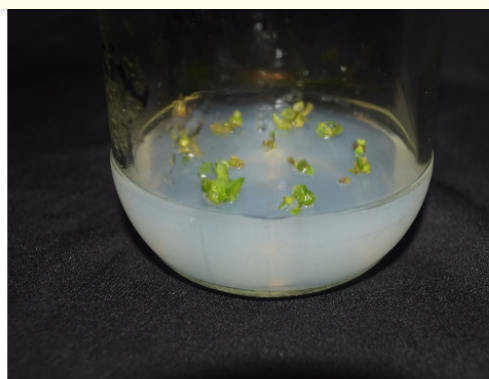
Photo 1: Shoot proliferation.
